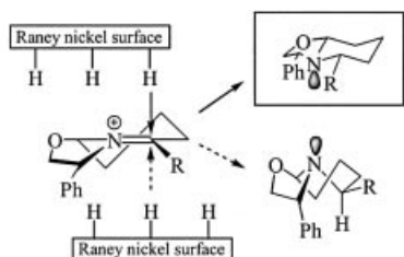
Figure 2. Mechanistic considerations for Raney nickel decyanation
