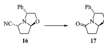
Scheme 6. Lactam formation in the pyrrolidine series; reagents and conditions: \text{KMnO}_4 (4 equiv.), acetone/ \text{H}_2\text{O} (1:1), room temp., 12 h (94%)
