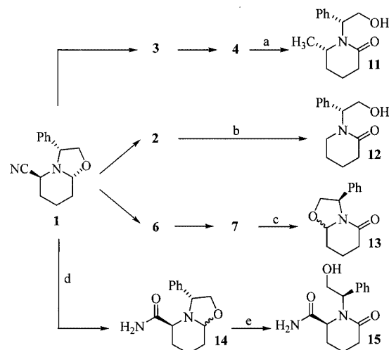
Scheme 5. Lactams derived from building block 1 ; reagents and conditions: (a) \text{KMnO}_4 (4 equiv.), acetone/ \text{H}_2\text{O} (7:3), room temp., 20 h (90%); (b) \text{KMnO}_4 (3 equiv.), acetone/ \text{H}_2\text{O} (1:1), room temp., 24 h (75%); (c) \text{KMnO}_4 (3 equiv.), acetone/ \text{H}_2\text{O} (1:1), room temp., 12 h (60%); (d) \text{H}_2\text{O}_2 (1.2 equiv.), \text{K}_2\text{CO}_3 , DMSO, 60 °C, 1 h (70%); (e) \text{KMnO}_4 (4 equiv.), acetone/ \text{H}_2\text{O} (1:1), room temp., 24 h (50%)
