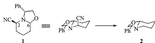
Scheme 1. Decyanation of building block 1 ; reagent and conditions: Raney nickel (excess), THF, reflux, 24–48 h (90%)
