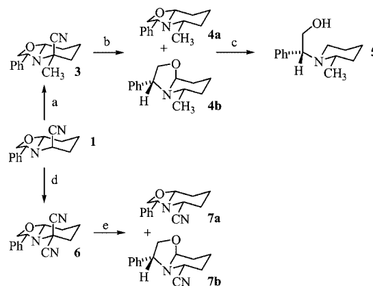
Scheme 2. Decyanation of building block 1 derivatives; reagents and conditions: (a) (i) LDA (3 equiv.), THF, -78^\circ\text{C} , 20 min, (ii) MeI (2 equiv.), -78^\circ\text{C} \rightarrow \text{room temp.} (95%); (b) Raney nickel (excess), THF, room temp., 1.5 h (quant., 4a/4b = 1.8); (c) \text{NaBH}_4 (5 equiv.), MeOH, room temp., 20 min (92%); (d) (i) LDA (3 equiv.), THF, -78^\circ\text{C} , 20 min, (ii) TsCN (2 equiv.), -78^\circ\text{C} , 4 h (67%); (e) Raney nickel (excess), THF, reflux, 3 h (20%, not optimized, 7b/7a = 3)
