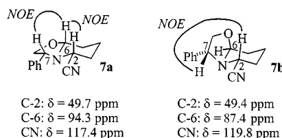
Figure 1. Selected NMR spectroscopic data for compounds 7a and 7b
