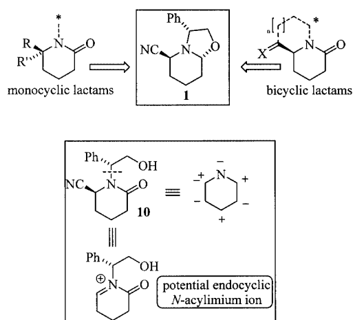
Figure 4. Lactams obtained from 1
