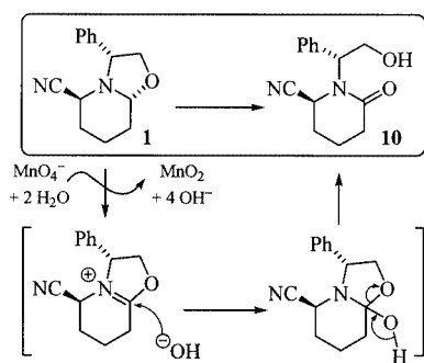
Scheme 4. Oxidation of building block 1 with potassium permanganate and plausible mechanism; reagents and conditions: \text{KMnO}_4 (7 equiv.), acetone/ \text{H}_2\text{O} (8:2), room temp., 2 d (80%)
