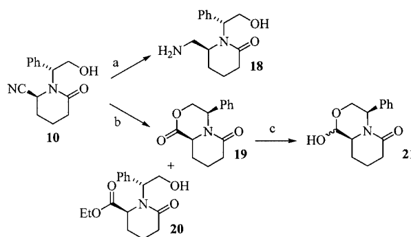
Scheme 7. Lactams derived from building block 10 ; reagents and conditions: (a) \text{H}_2 (11 bar), \text{PtO}_2 (1 equiv., w/w), EtOH, room temp., 5 d (70%); (b) \text{HCl} /EtOH, room temp., 20 d ( 19 : 65%; 20 : < 5%, conversion 80%); (c) \text{NaBH}_4 (1.2 equiv.), MeOH, room temp., 30 min (93%)
